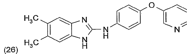
(5,6-Dimethyl-1H-benzimidazol-2-yl)-[4-(pyridin-3-yloxy)-phenyl]-amin
